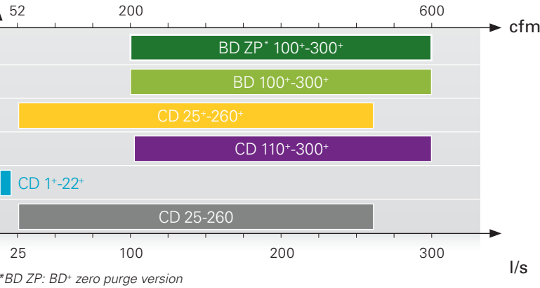
Atlas Copco desiccant dryer range
